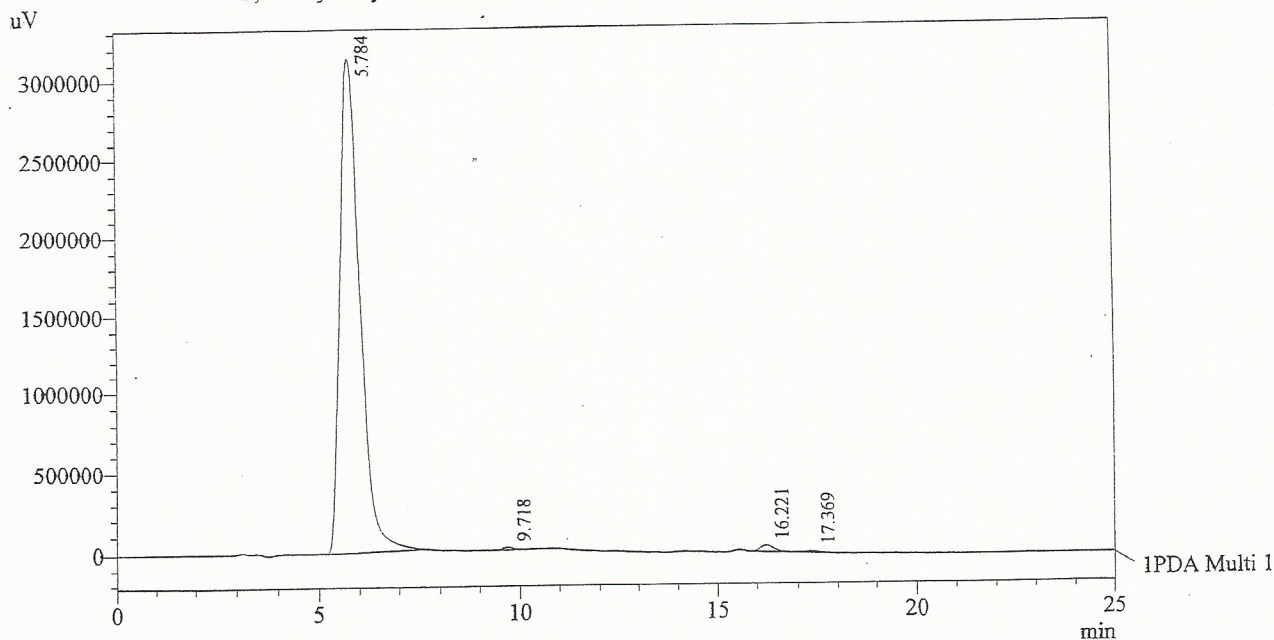
Chromatogram 3,4-Dihydroxy benzoic acid monohydrate D:\promonence\2010\Feb-10\040210C.lcd
